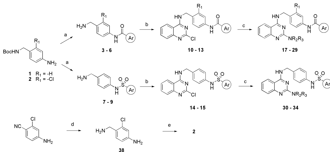
Scheme 1 a
