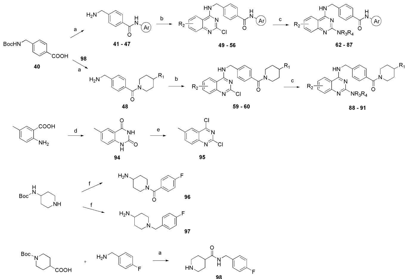
Scheme 2 a
